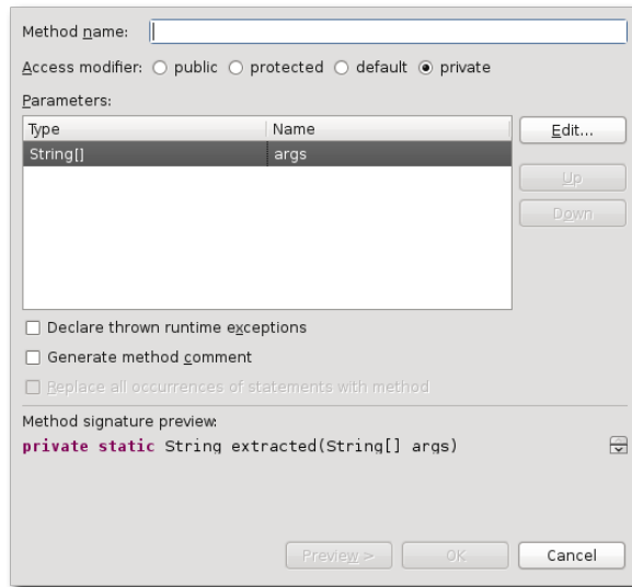
Figure 3.8.: Eclipse JDT's Extract Method Refactoring can be highly customized.
