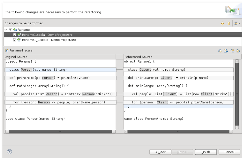
Figure 3.2.: A classical Rename refactoring: All occurrences of the selected name are changed across all files in the project.
