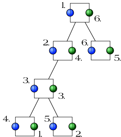
Figure 2.5.: An illustration of the pre- and post-order traversal strategies: the blue points show the order in which the tree gets transformed in pre-order traversal, and the green ones illustrate the post-order traversal. Instead of pre- and post-order, we can also think of the transformations being applied top-down or bottom-up, hence the \downarrow and \uparrow aliases.
